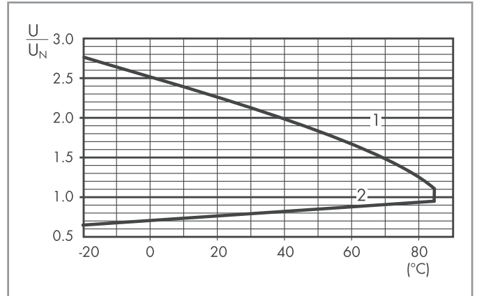
R 36 - DC coil operating range v ambient temperature
